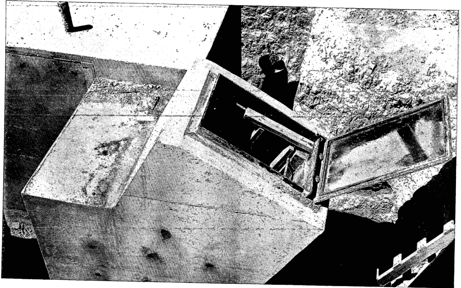
Fig. 4—Shelter entrance corridor before backfill.
